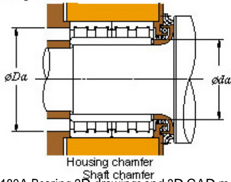
44FC34180A Bearing 2D drawings and 3D CAD models
